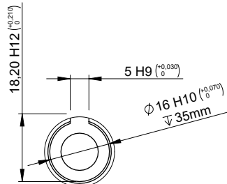
Input shaft detail Scale 1:1
