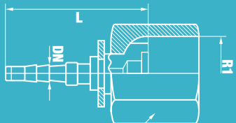
1/4" BSP
