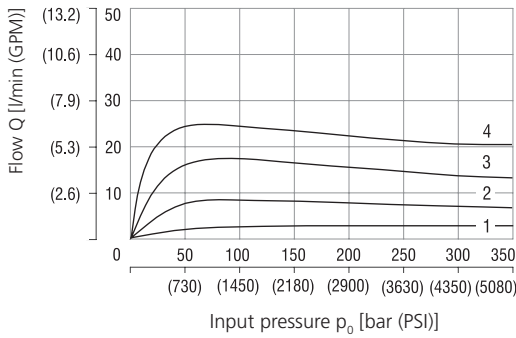
Regulated flow related to control signal \Delta p = 10 \text{ bar} (145 PSI)
