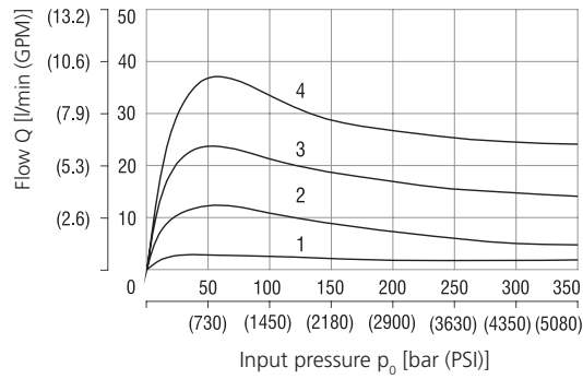
Nominal flow 30 l/min (7.9 GPM)
