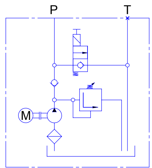
Hydraulic Circuit P, T = G 3/8
